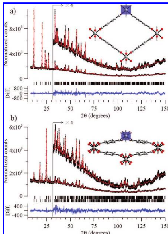
Figure 1. Neutron powder diffraction data (black points) of MIL-53(Al) collected at room temperature after heating to 450 K (upper) and cooling to 77 K (lower). MIL-53(Al) exists either as an open-pored (HT) phase or a predominantly closed-pored phase (LT), depending on the thermal history. The solid red lines are Rietveld refinement fits to the data using the structural models given in the text and illustrated in the inset. Vertical markers give Bragg peak positions for the respective phases and the solid line beneath is the difference between the experimental and calculated intensities. Note the scaling factor applied to the upper patterns and the difference data for angles greater than 26^\circ . Error bars in the experimental data indicate one standard deviation of the counting statistics.
