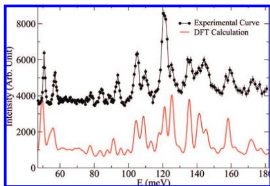
Figure 5. Comparison of the high energy inelastic neutron scattering data for MIL-53(Al) in the LT phase (circles) and that predicted from the DFT calculation (solid line). Data are displaced for clarity. Error bars for the experimental data indicate one standard deviation of the counting statistics.
